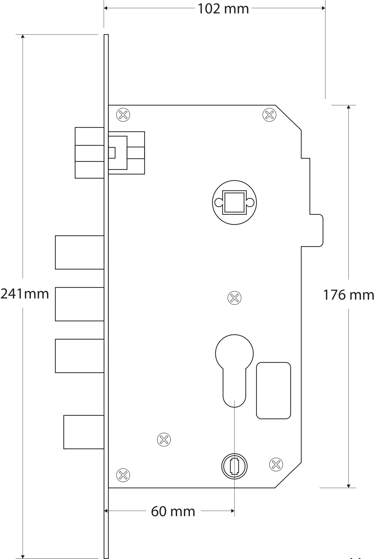
Mortise DDL603 (60mm)
