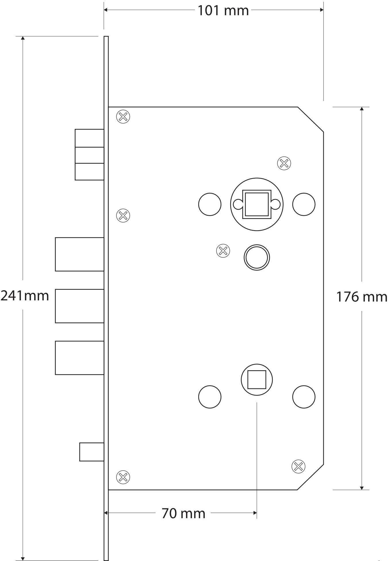
Mortise DDL709 (70mm)
